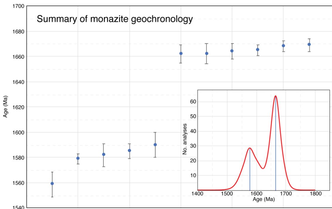
Figure 22: Summary of monazite geochronology from this study. Mean ages from the geochronological populations in the samples are plotted in age order with 2σ error bars. Two distinct ages are present at ca. 1670 – 1660 Ma and ca. 1590 – 1580 Ma. Sample SFDD01-09 yields a younger mean age at 1559 Ma. Inset: age probability plot highlighting the statistical significance of the two older ages.
