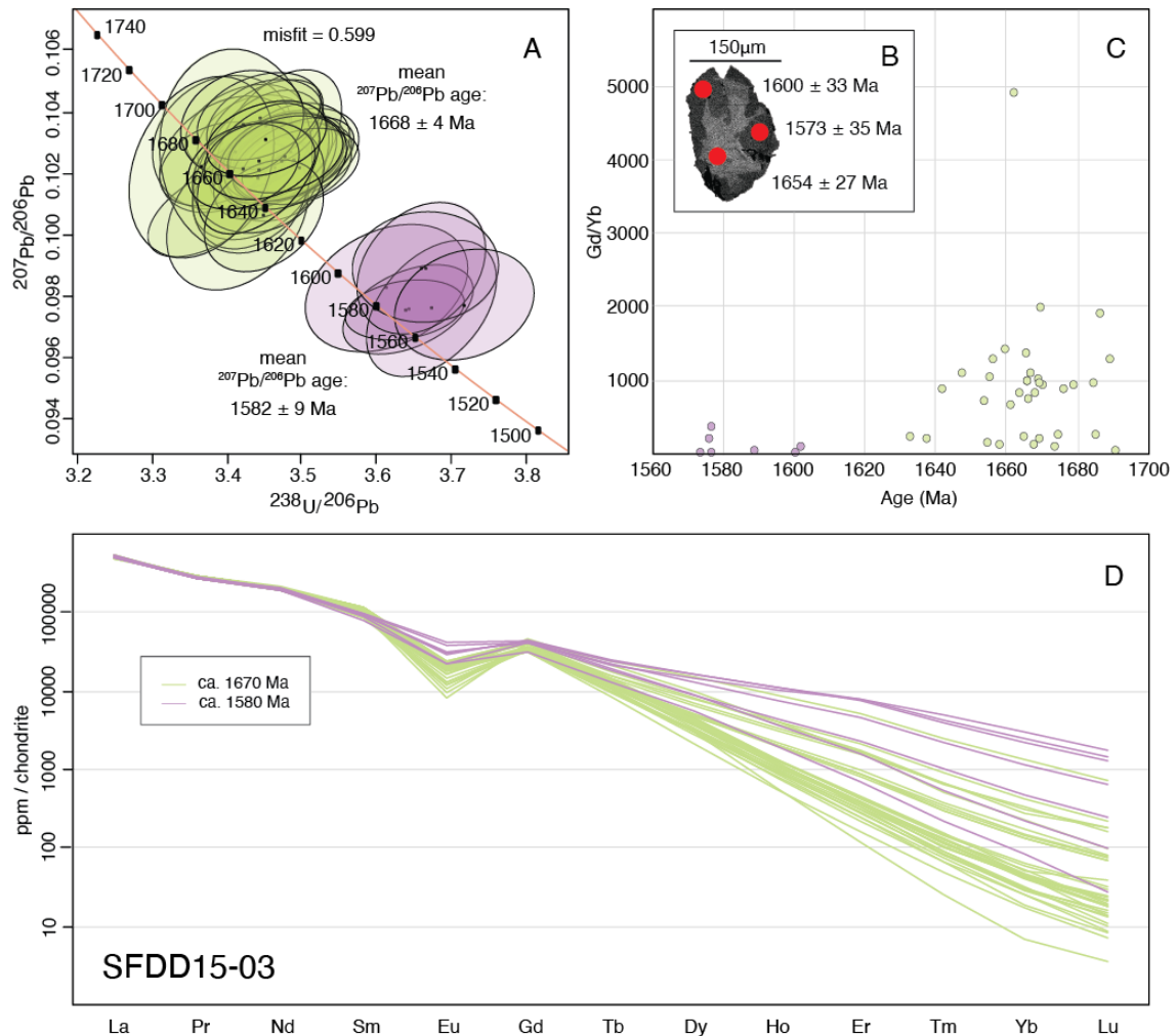
Figure 16: Monazite LA-ICP-MS results for sample SFDD15-03. (a) Terra-Wasserburg concordia plot with 2 sigma error ellipses. Ages are given in Ma. Concordant data yields two ages of 1668 \pm 4 Ma and 1582 \pm 9 Ma with a relative misfit of 0.599. The spots are coloured by age population. (b) BSE image of a monazite grain. The grain has an older core with a younger rim. (c) Gd/Yb ratios for concordant analyses show that the younger analyses are comparatively enriched in HREEs
